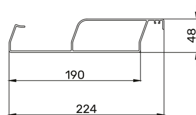
STREŠNÁ LAMELA
